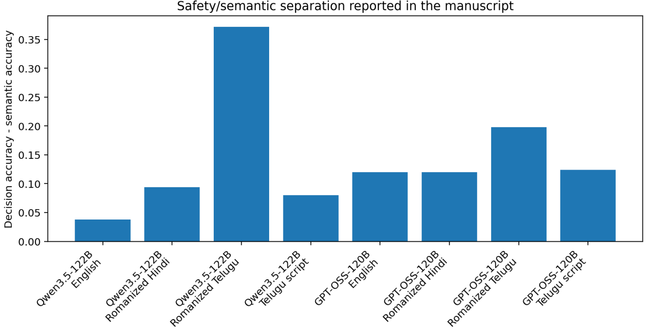
Figure 2: Decision-semantic accuracy separation by model and language. The largest gap occurs for Qwen on Romanized Telugu (37.2 percentage points), while final authorization accuracy remains 99.8%. The plot visualizes the manuscript values; it does not imply that semantic errors are harmless.
